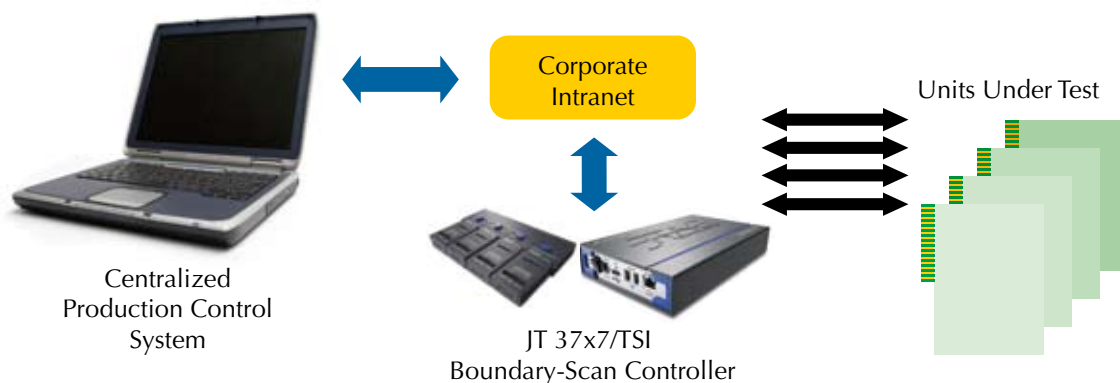
Figure 2. Block diagram of TSI-based remote operation
