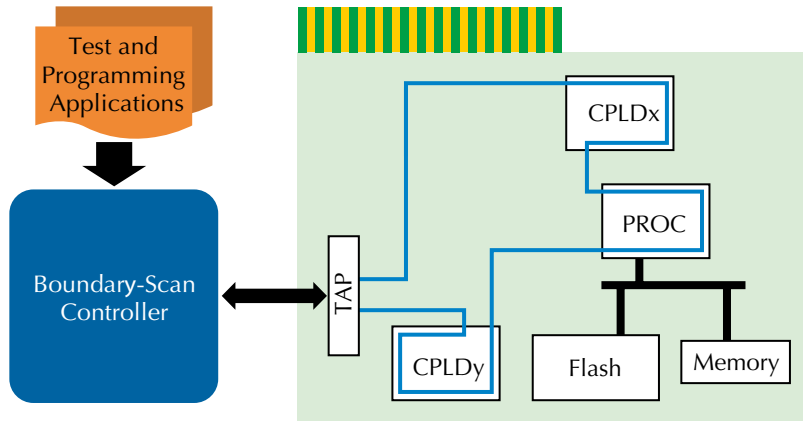
Figure 1. Block diagram
